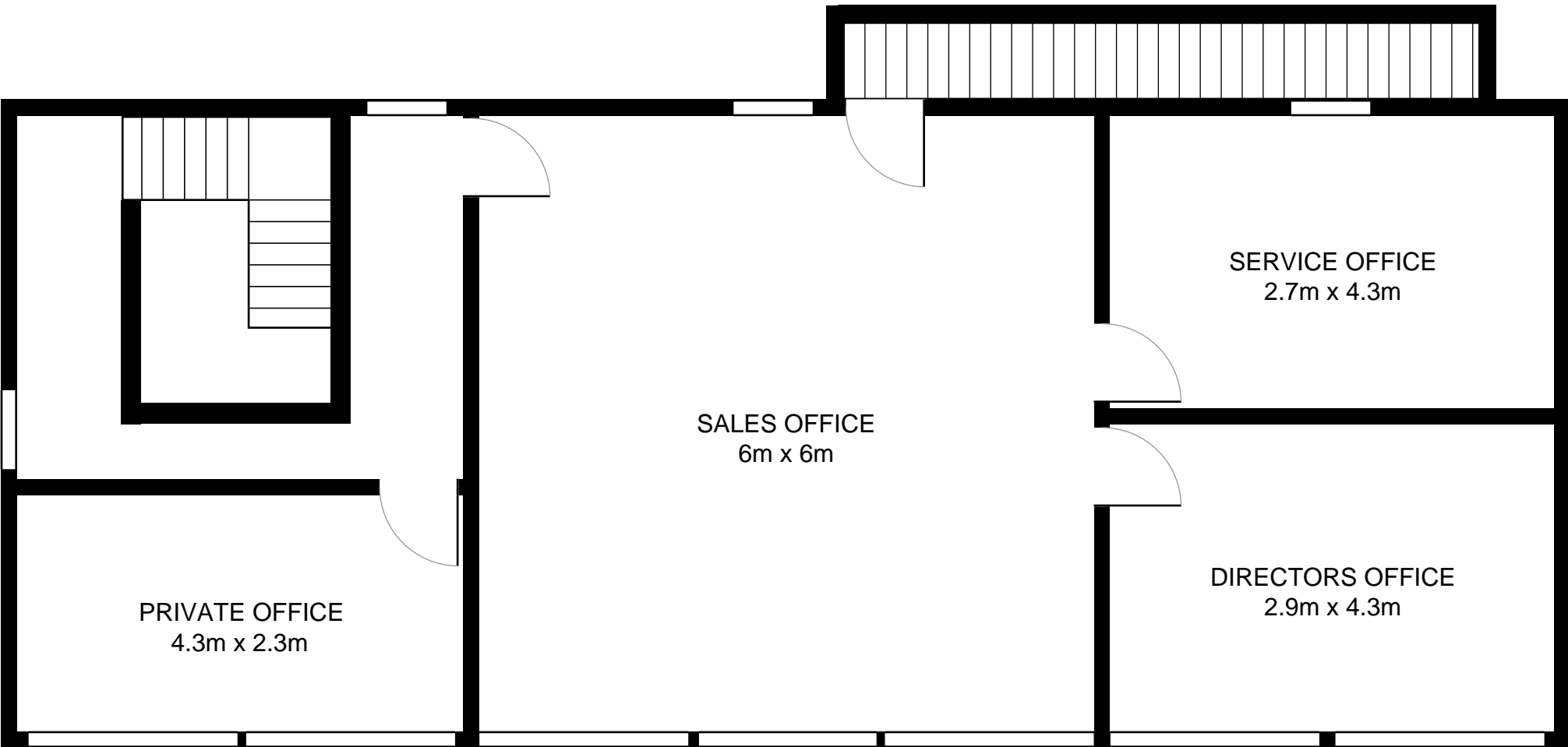
FIRST FLOOR
